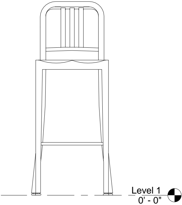
① Front View 1" = 1'-0"
