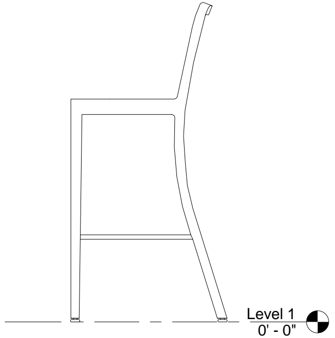
② Side View 1" = 1'-0"
